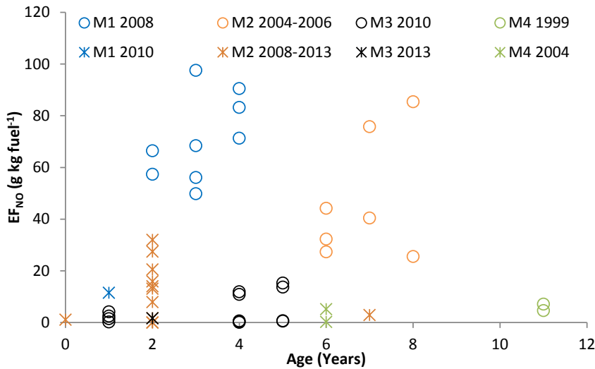
Figure 3 EF NO from methane powered buses by manufacturer, model year and age.
